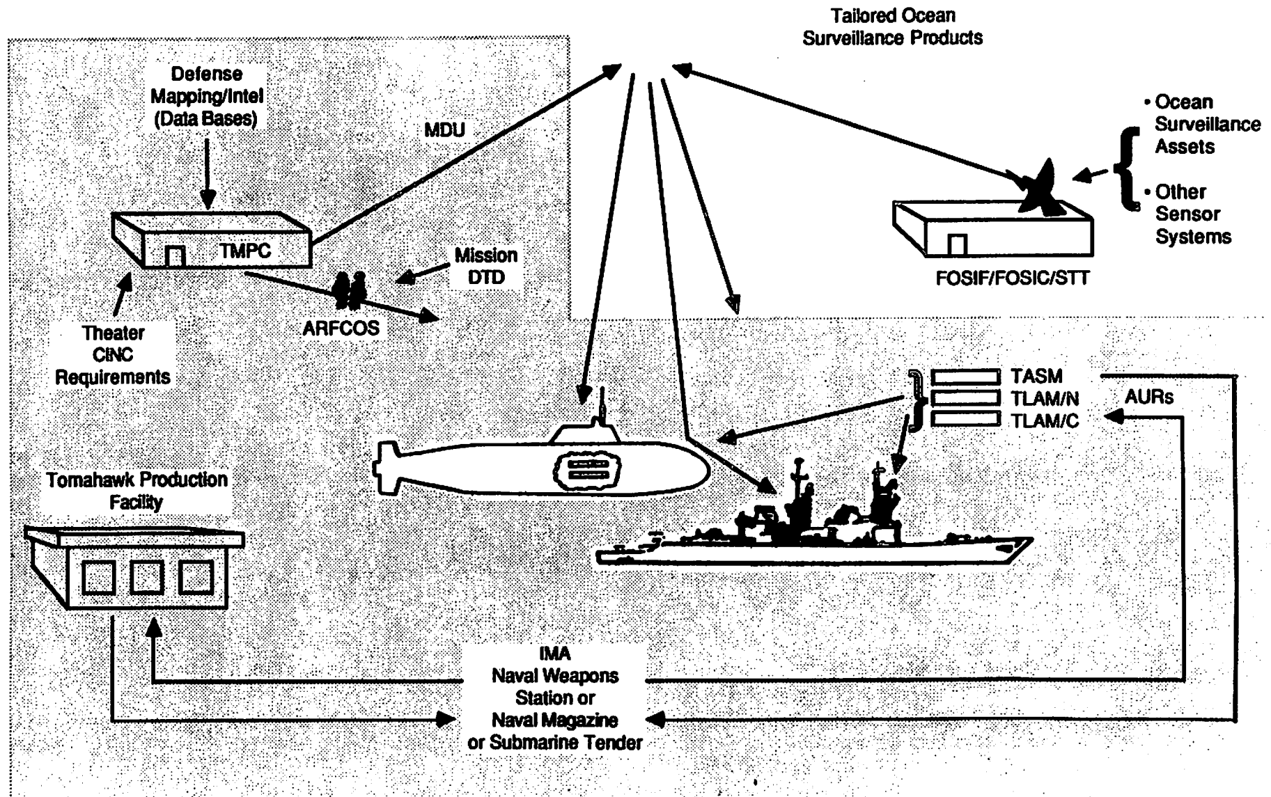
Figure D-4 Tomahawk Integrated Weapon System "Except for Sensors and C2"
